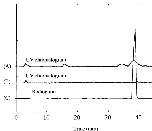
Figure 1. Radiogram and ultraviolet chromatograms to document the radiochemical and chemical purity of compound 6i . (A): UV chromatogram of a mixture of 6f and 6d ; (B) and (C): Radiogram and UV chromatogram of 6i after HPLC purification.
