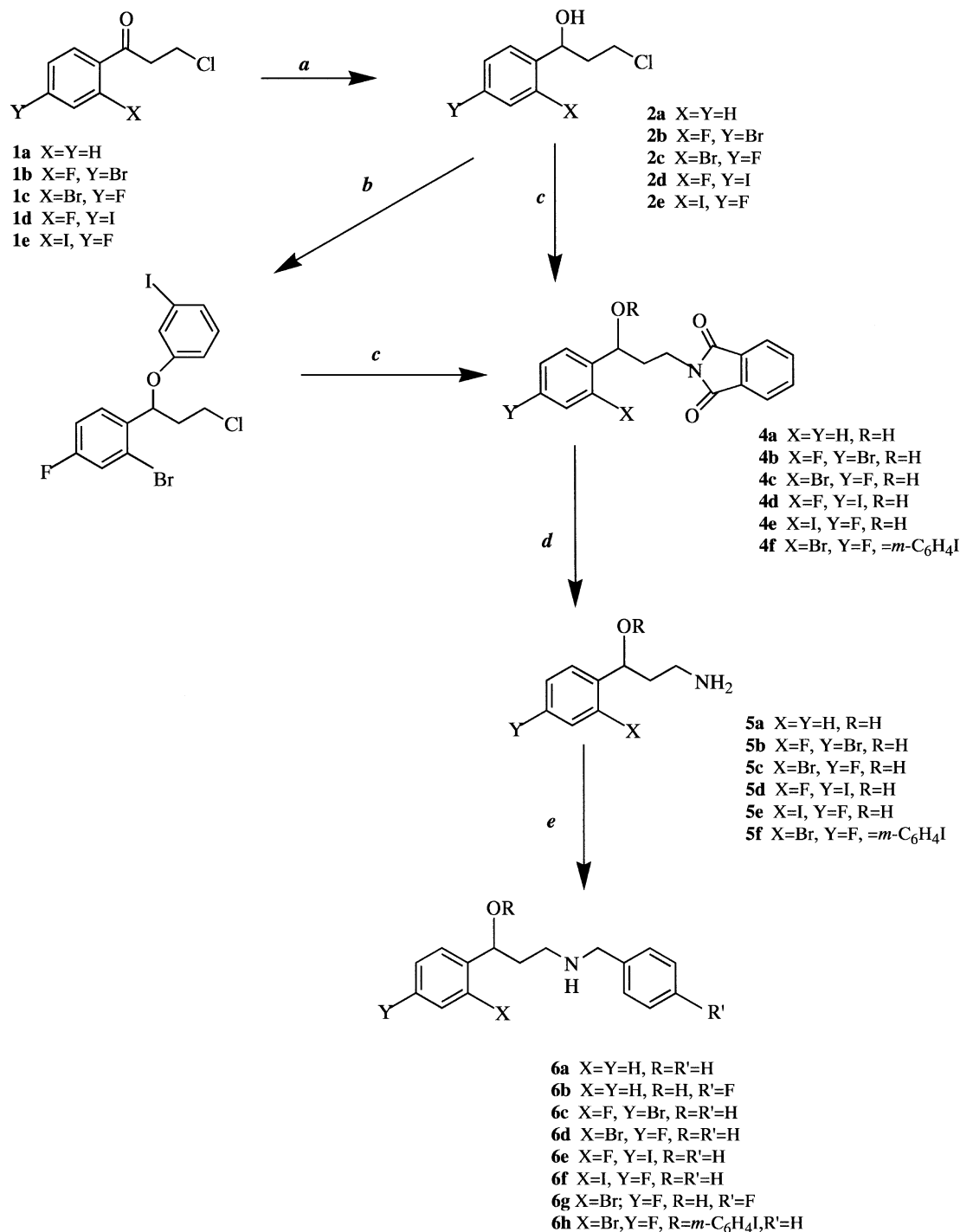
Scheme 1. Preparation of aminoalcohols 6a–6h : (a) NaBH 4 in CH 3 OH at 0 °C; (b) 3-iodophenol, DEAD/PPh 3 in THF, 21 h at rt; (c) phthalimide and anhydrous KF in DMF at 120 °C for 8 h; (d) hydrazine in H 2 O/CH 3 OH/HCl, reflux, 3 h; (e) benzaldehyde or p -fluorobenzaldehyde, NaBH 3 CN in CH 3 OH, 24 h at rt.
