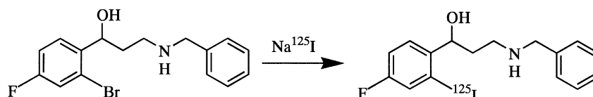
Scheme 2. Preparation of aminoalcohol 6i : Na 125 I, Cu(I)-organo complexes in EtOH–H 2 O, 100 °C, 90 min.
