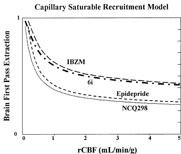
Figure 2. First pass cerebral extraction (experimental data fitting based on the capillaries recruitment model) of compound 6i , IBZM, Epidepride and NCQ298.
